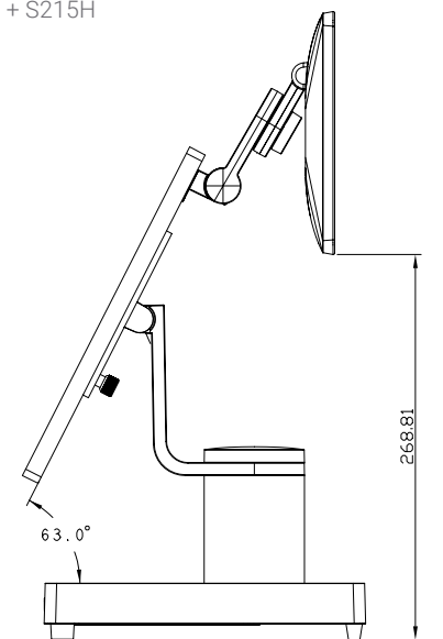
VariPOS S150 + M135 ( Triple-Hinge )
