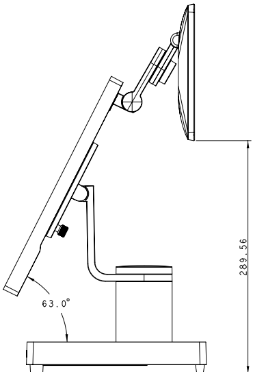
VariPOS S215 + M135 ( Triple-Hinge )
