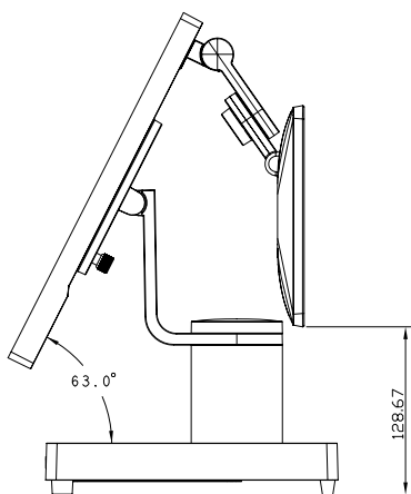
VariPOS S215 + M135 ( Triple-Hinge )
