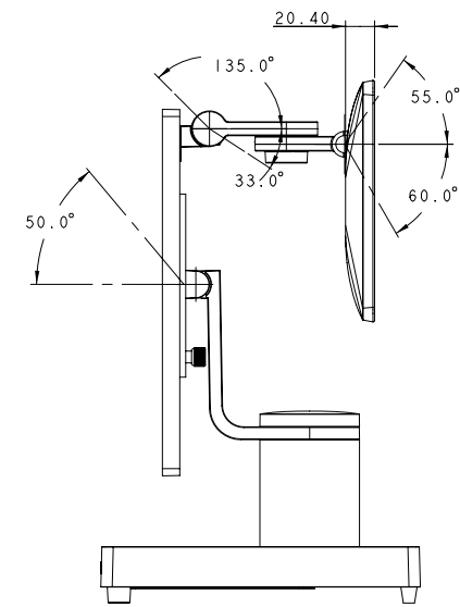
VariPOS S150 + M135 ( Triple-Hinge )
