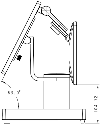
VariPOS S156 + M135 ( Triple-Hinge )
