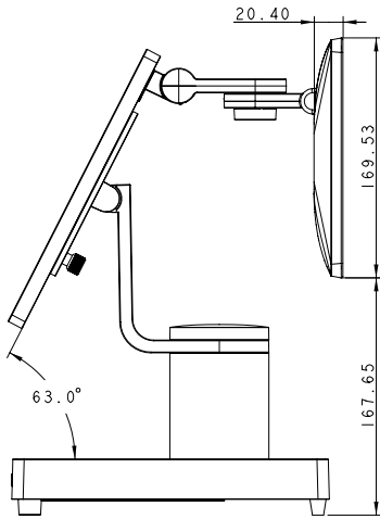
VariPOS S156 + M135 ( Triple-Hinge )
