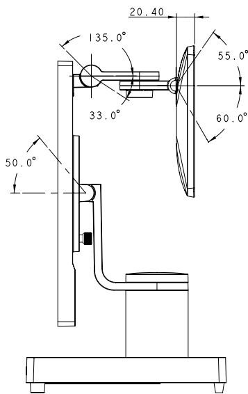
VariPOS S215 + M135 ( Triple-Hinge )
