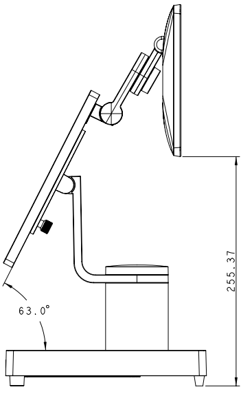
VariPOS S156 + M135 ( Triple-Hinge )
