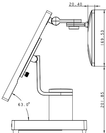
VariPOS S215 + M135 ( Triple-Hinge )
